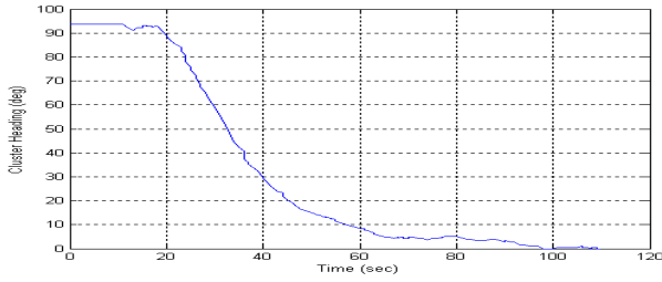
(b) Time history of cluster heading given a desired value of \theta_c = 0^\circ at t = 10 sec.
