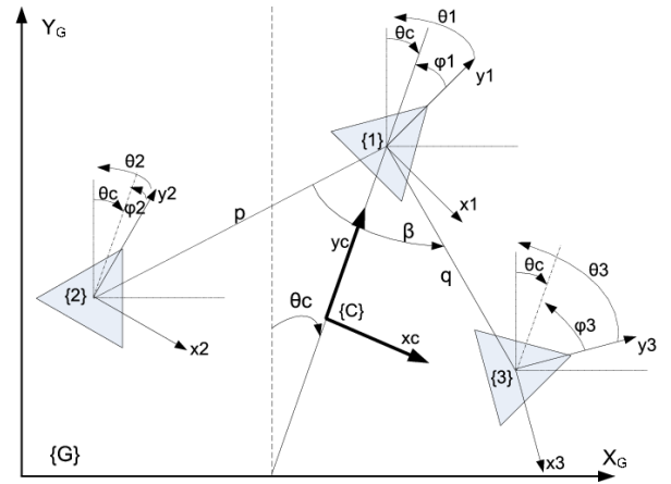
Fig. 4 – Pose reference frames for the planar 3-robot system
