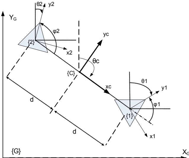
Fig. 3 – Pose reference frames for the planar 2-robot system
