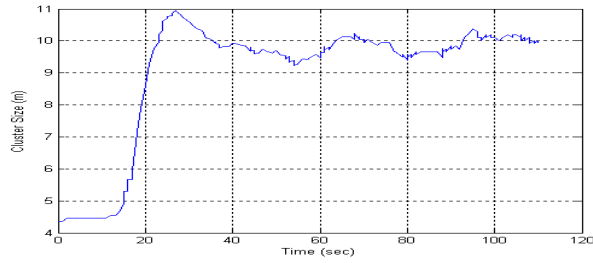
(c) Time history of cluster size given a desired value of d = 10 m at t = 10 sec.
