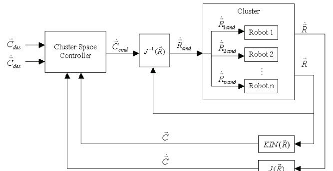
Fig. 2 – Cluster Space Control Architecture for a Mobile Multi-Robot System. In this cluster space control architecture, desired motions and control actions are computed in the cluster space; control actions are converted to the robot space through the use of the inverse Jacobian relationship.
